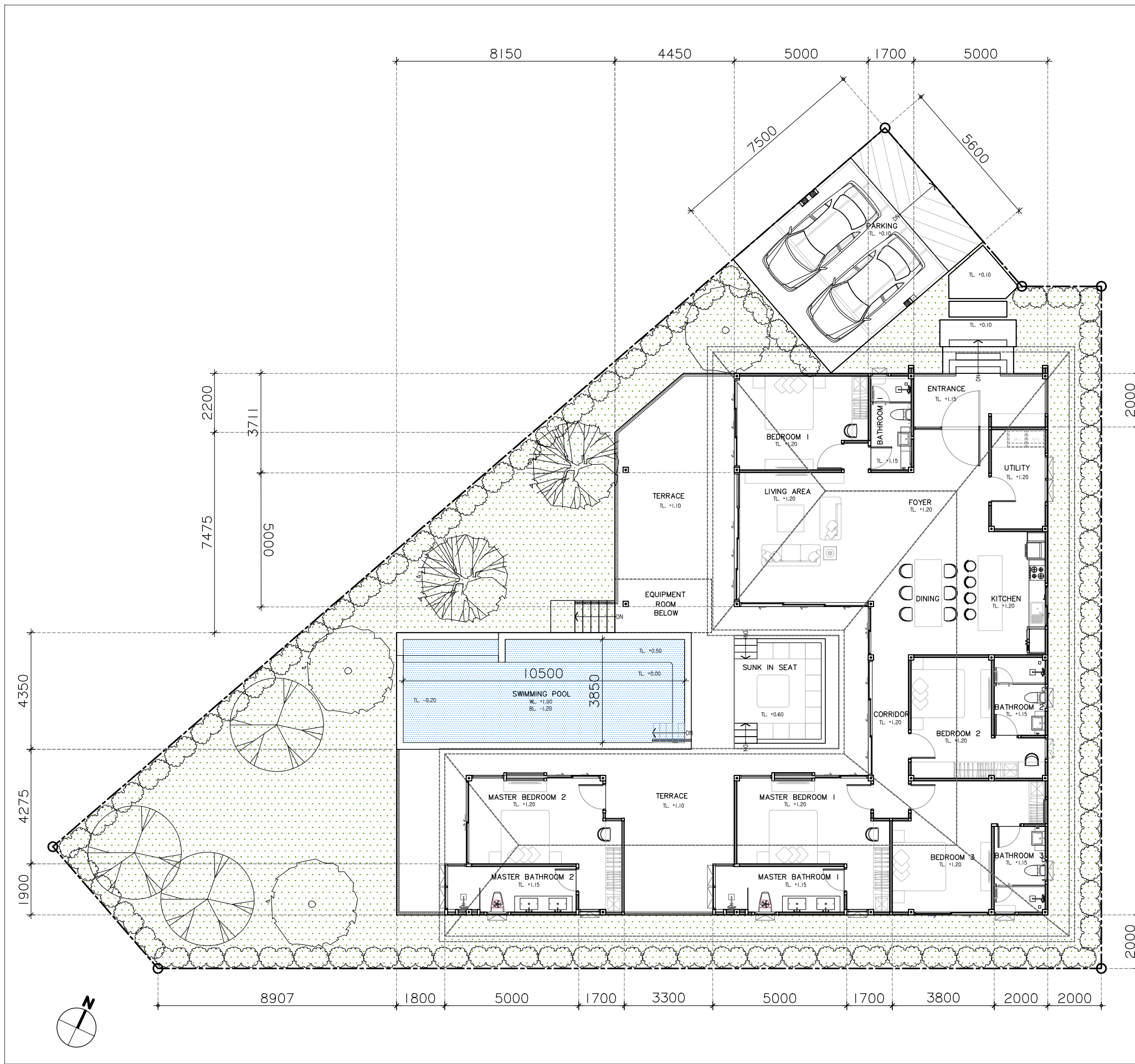
FLOOR PLAN 5 BEDROOMS PLOT : K21 ISSUE DATE 2025-04-25
